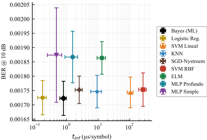
BER vs Inference Latency Trade-off
